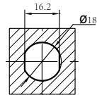
Steel cabinet mounting hole size
